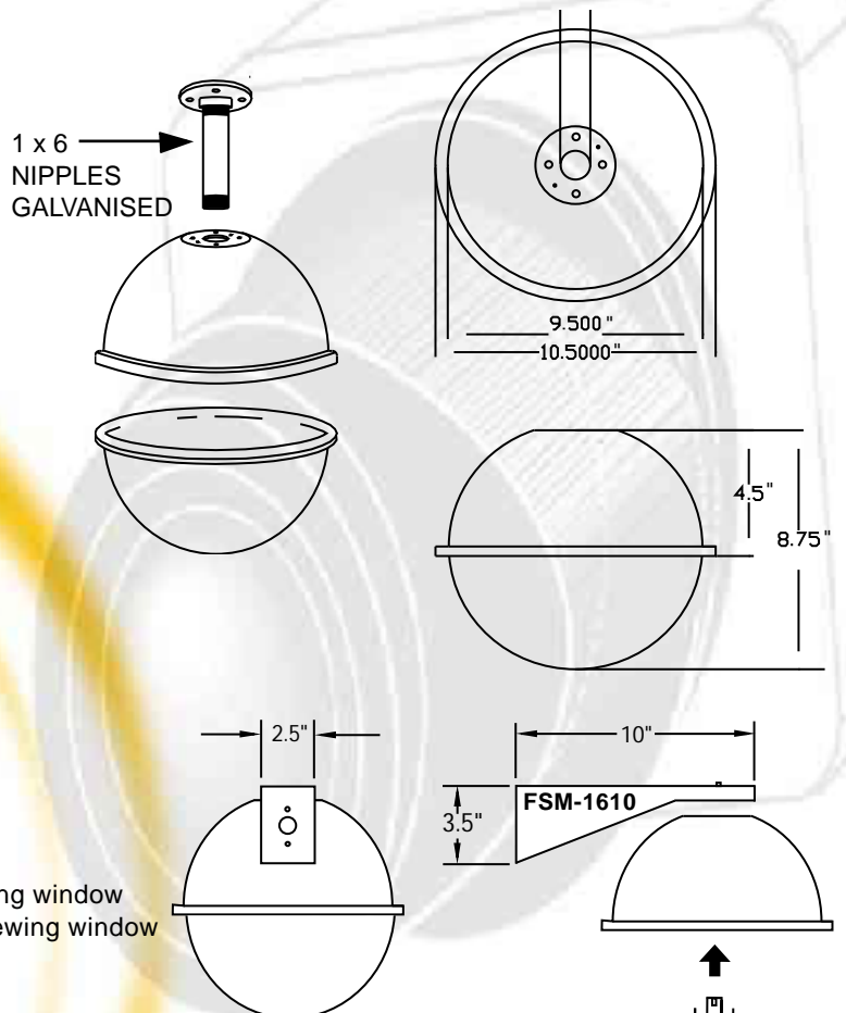
Shown with optional FS-0032 for camera board
